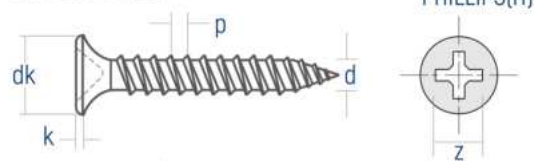
Twinfast thread
